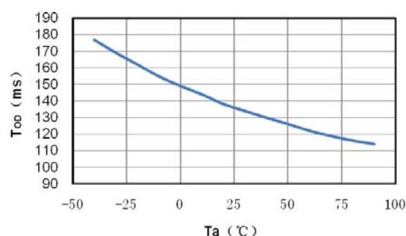
(6) T_{OD} vs. T_a
