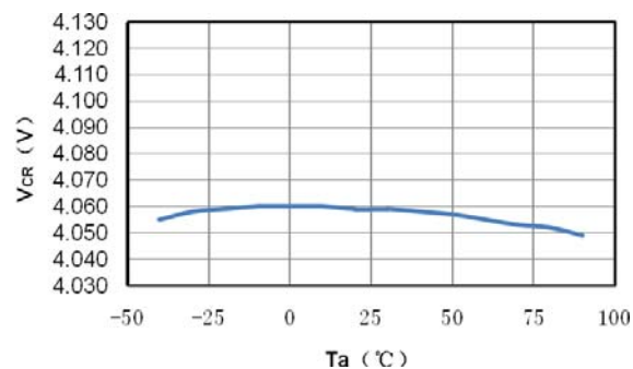
(2) V_{CR} vs. T_a
